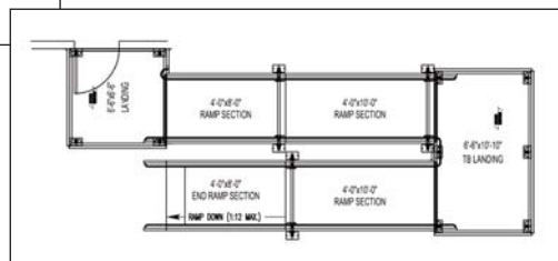
Below - Ramp with stair system footprint. Additional stairs can be added to the system.
