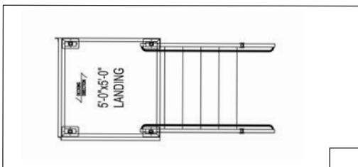
Above - Landing and stair footprint. Stairs can be installed on either one of the three available sides.
