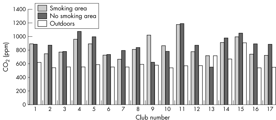
Figure 3 Concentration of atmospheric CO 2 in clubs: smoking versus "no smoking" and outdoor areas.
